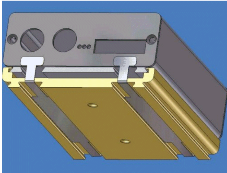
Figure 1A – DVMD1/1X Mounting Base (Gold and Silver) CAD Drawing
